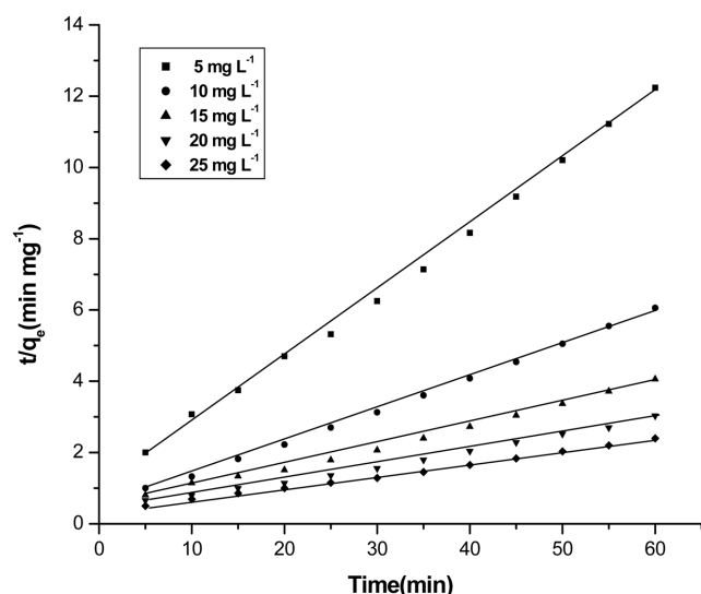
Figure 5. Second-order kinetic model plot for different concentrations of iron. Conditions are solution pH: 6.0, solution temperature: 305 K, and current density: 0.06\text{ A dm}^{-2} .
