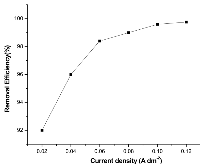
Figure 2. Effect of current density on the removal of iron. Conditions are solution pH: 6.0, concentration of iron: 25 \text{ mg L}^{-1} , and solution temperature: 305 K.
