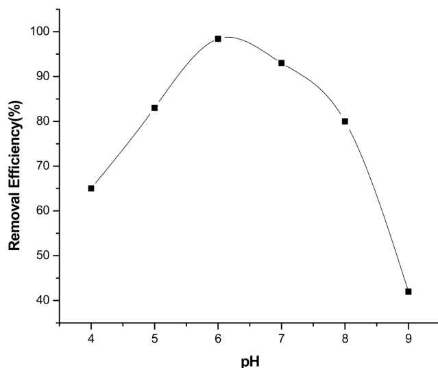
Figure 3. Effect of pH on the removal of iron. Conditions are concentration of iron: 25 \text{ mg L}^{-1} , current density: 0.06 \text{ A dm}^{-2} , and solution temperature: 305 K.
