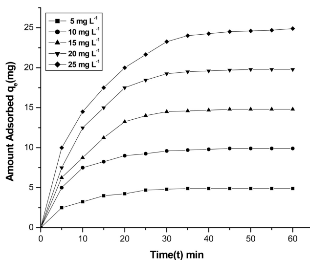
Figure 4. Effect of agitation time and initial iron concentration on the amount of iron adsorbed. Conditions are solution pH: 6.0, solution temperature: 305 K, and current density: 0.06 \text{ A dm}^{-2} .
